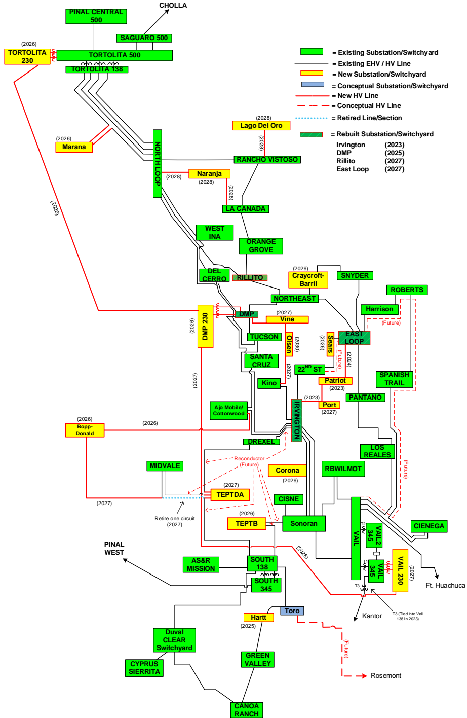
Figure 4: TEP Local Area HV Ten Year Transmission Plan
