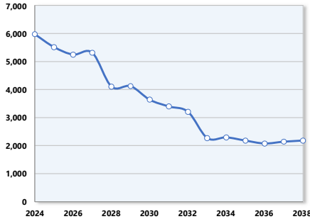
CO 2 Emissions, Thousand Metric Tons
