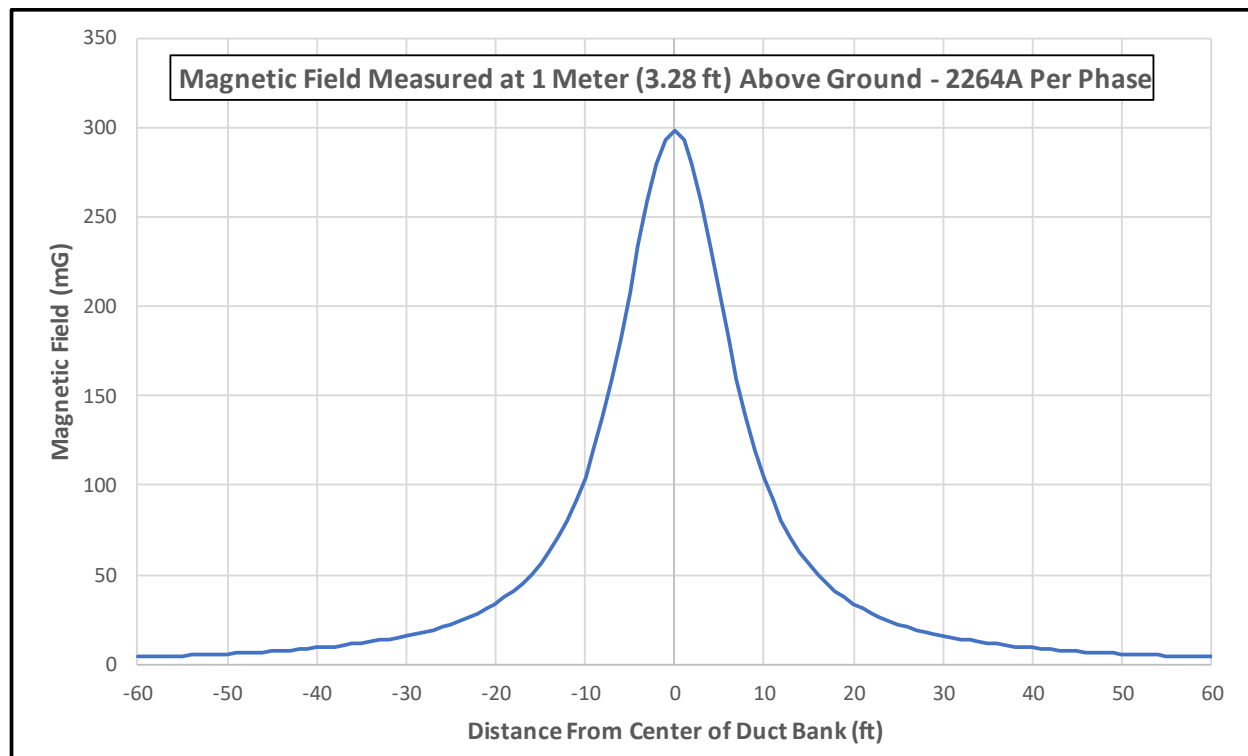
Figure 3-2 – 2264A Per Phase Magnetic Field Results
