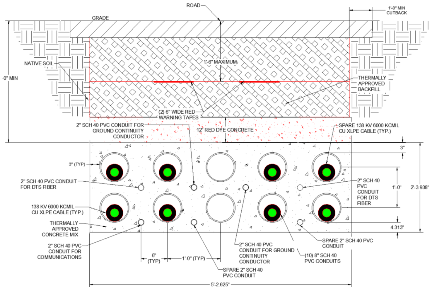
Figure 3-3 — Preliminary Duct Bank Layout
