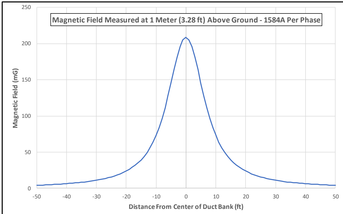
Figure 3-1 – 1584A Per Phase Magnetic Field Results
