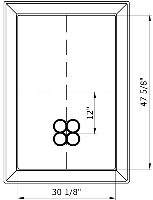
SECONDARY JUNCTION BOX (J-30) TOP VIEW
