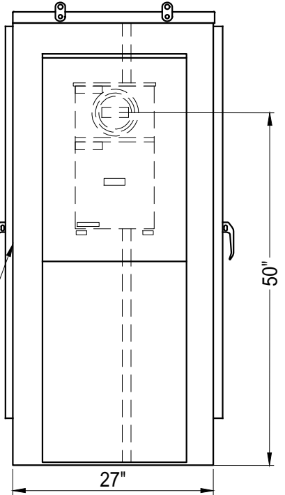
SIDE VIEW METER ENCLOSURE
