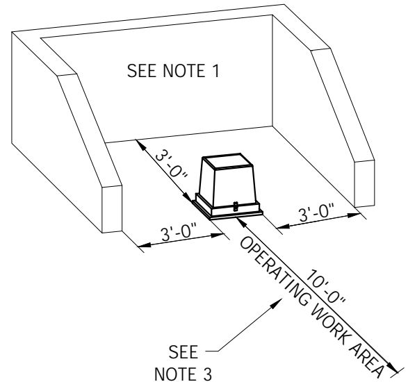
FIGURE 7 PEDESTAL, J10 OR J30 CLEARANCE
