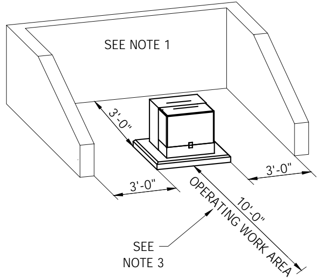
FIGURE 6 TRANSFORMER CLEARANCE
