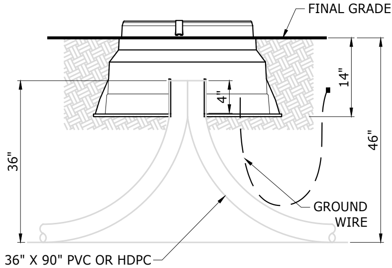
SECONDARY PEDESTAL FRONT VIEW
