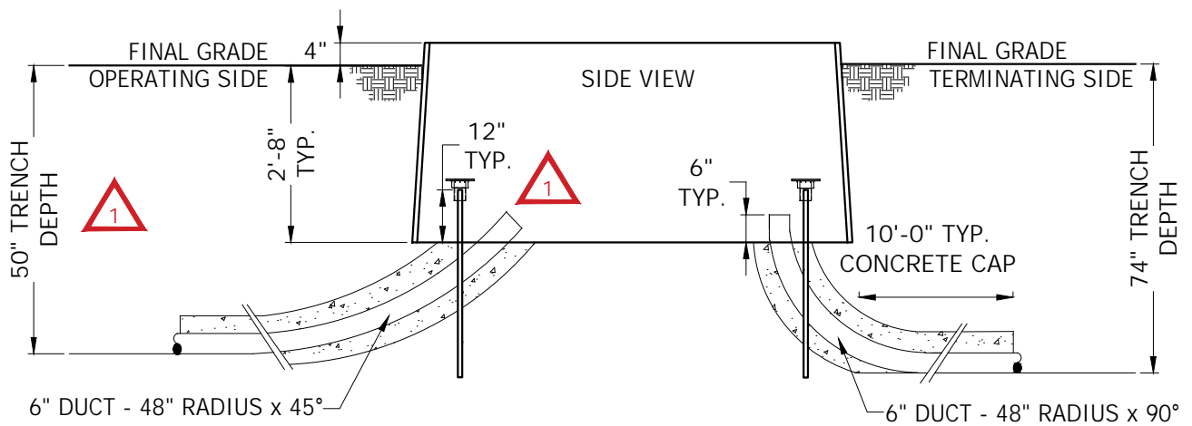
DUCT LOCATION WHEN LEAVING TOWARD STREET/ALLEY/UTILITY EASEMENT
