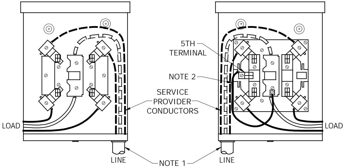
FIGURE 1 120/240V, 3W, 1Ø
