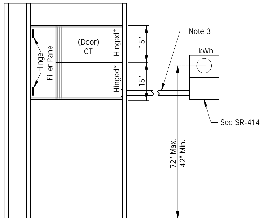
TYPICAL INSTALLATION
