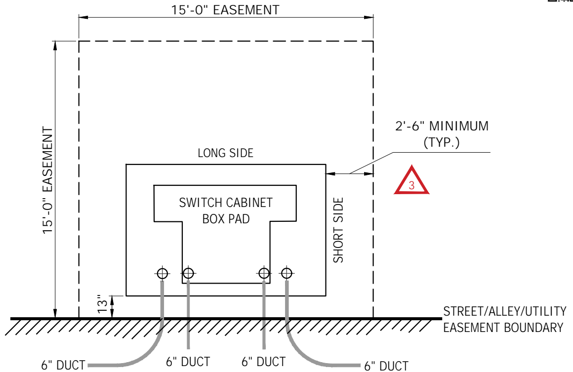
EQUIPMENT PLACEMENT IN TYPICAL EASEMENT
